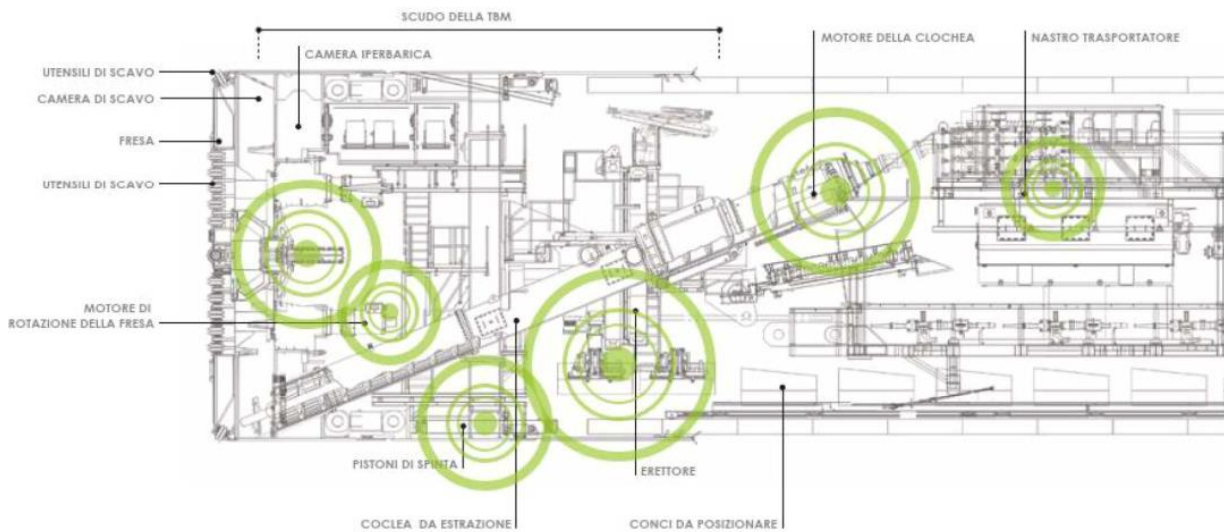
Figura 10-5.: Energy efficiency points of a "Green" TBM
